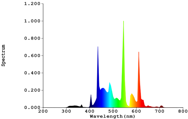
13W CFL Lamp UVB 2.0
