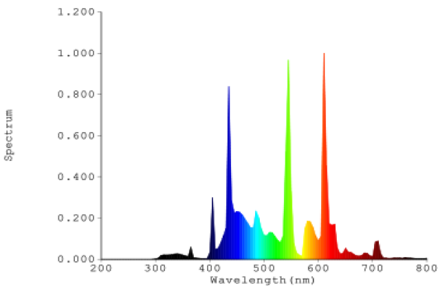
26W CFL Lamp UVB 2.0
